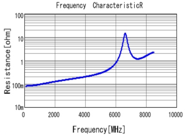
GJM1555C1H100JB01 R DC0V, 25degC
