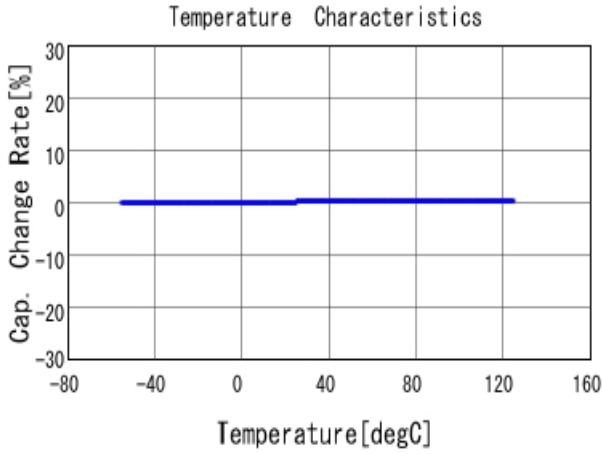
GJM1555C1H100JB01 C-Temp. capchange, DCOV, AC1Vrms
