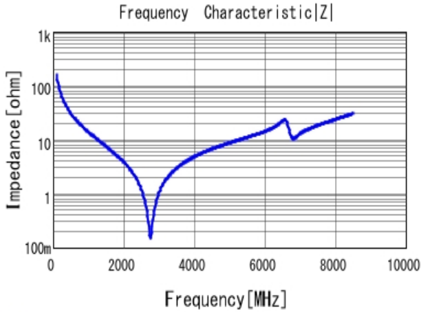
GJM1555C1H100JB01 |Z| DC0V, 25degC
