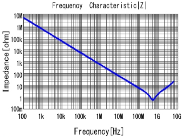
■ GRM155R72A331KA01 |Z| DCOV, 25degC
