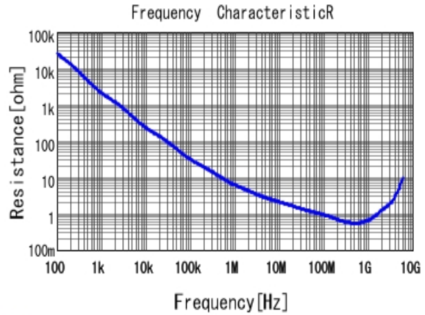
■ GRM155R72A331KA01 R DCOV, 25degC
