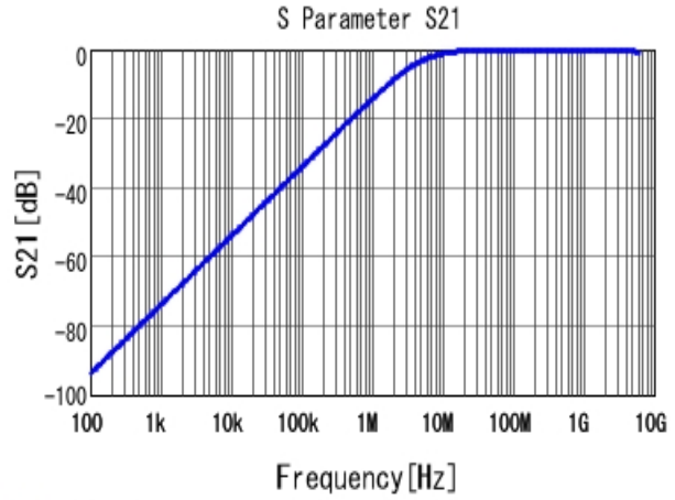
■ GRM155R72A331KA01 S21 DCOV, 25degC
