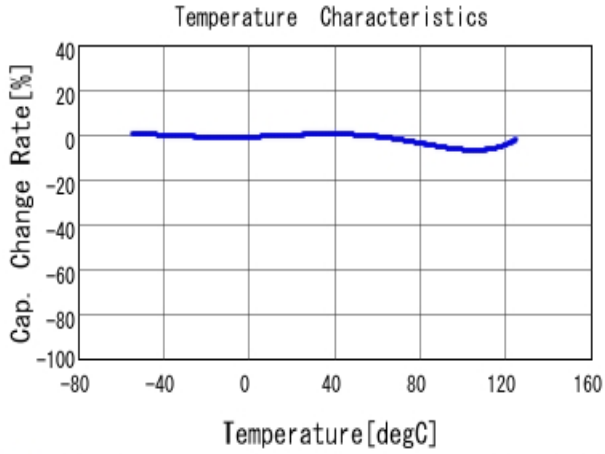
■ GRM155R72A331KA01 C-Temp. capchange, DCO. 0V, AC1.0Vrm
