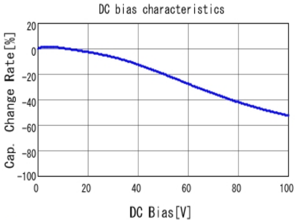
■ GRM155R72A331KA01 C-DC bias capchange, 25.0degC, AC1.
