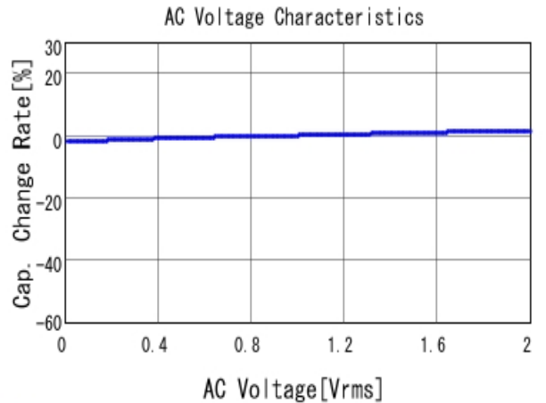
■ GRM155R72A331KA01 C-AC Voltage capchange, DCOV, 25.0d
