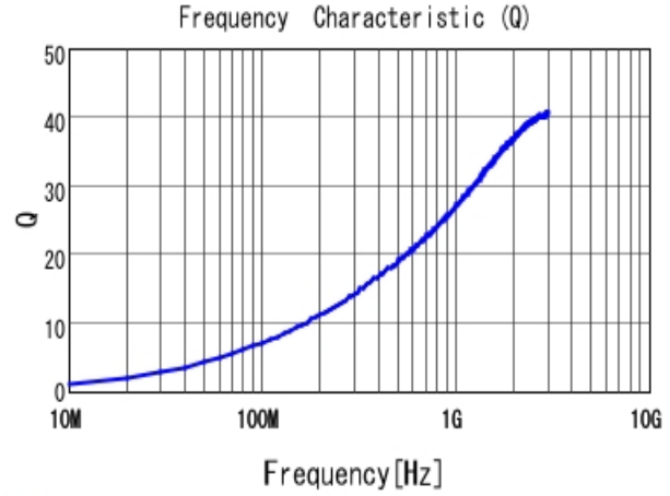
■ LQP15MN3N4W02 Q
