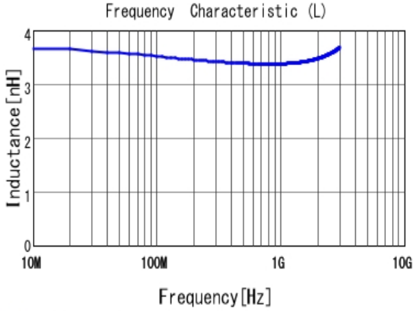
■ LQP15MN3N4W02 L
