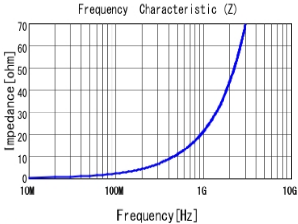
■ LQP15MN3N4W02 |Z|
