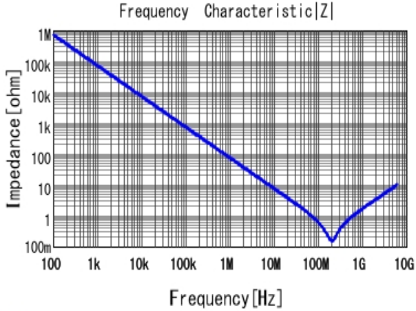
GCM033R71C222KA55 |Z| DC0V, 25degC
