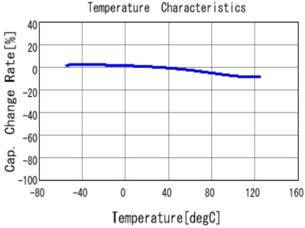
■ GCM033R71C222KA55 C-Temp. capchange, DC0.0V, AC1.0Vrm
