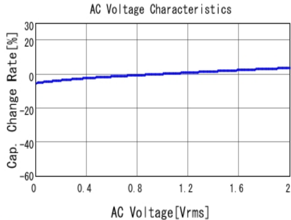
GCM033R71C222KA55 C-AC Voltage capchange, DC0V, 25.0d
