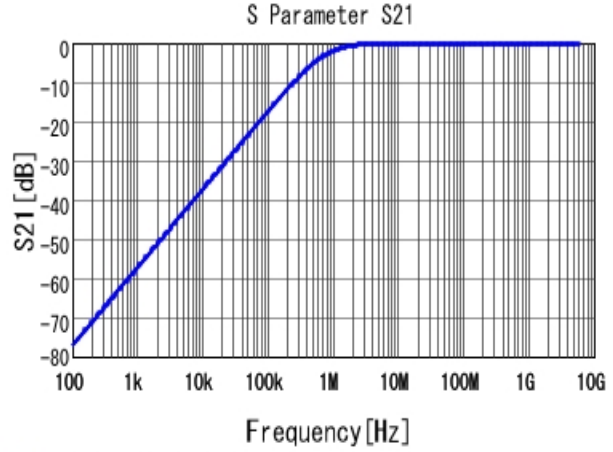
■ GCM033R71C222KA55 S21 DC0V, 25degC
