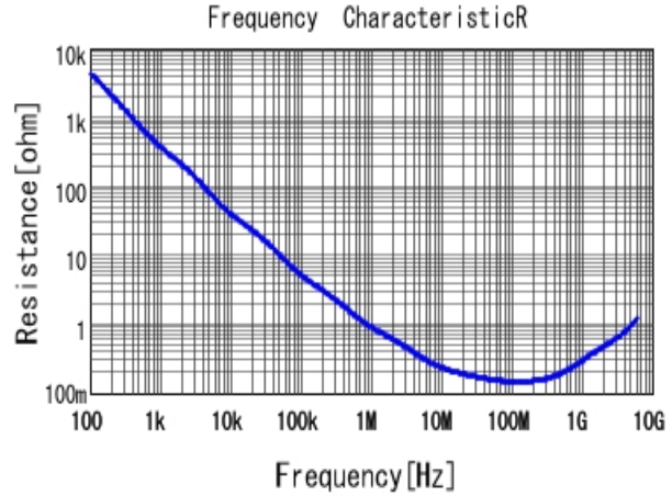
GCM033R71C222KA55 R DC0V, 25degC
