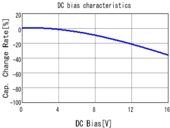
GCM033R71C222KA55 C-DC bias capchange, 25.0degC, AC1.
