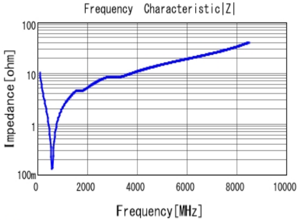
■ GRM2165C2A151JA01 |Z| DCOV, 25degC
