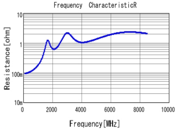
■ GRM2165C2A151JA01 R DCOV, 25degC
