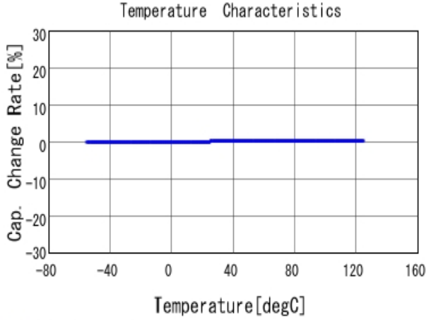
■ GJM0335C1E3R1BB01 C-Temp. capchange, DCOV, AC1Vrms
