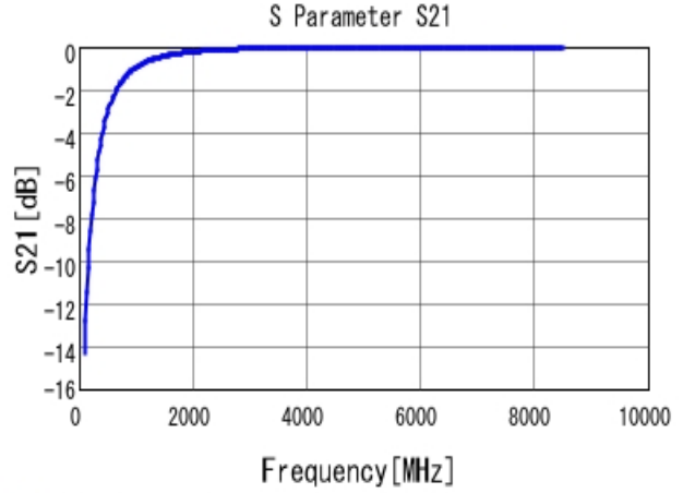
■ GJM0335C1E3R1BB01 S21 DCOV, 25degC
