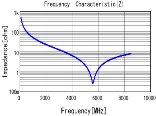
GJM0335C1E3R1BB01 |Z| DC0V, 25degC
