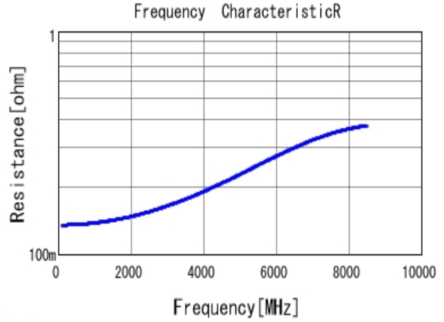
GJM0335C1E3R1BB01 R DC0V, 25degC
