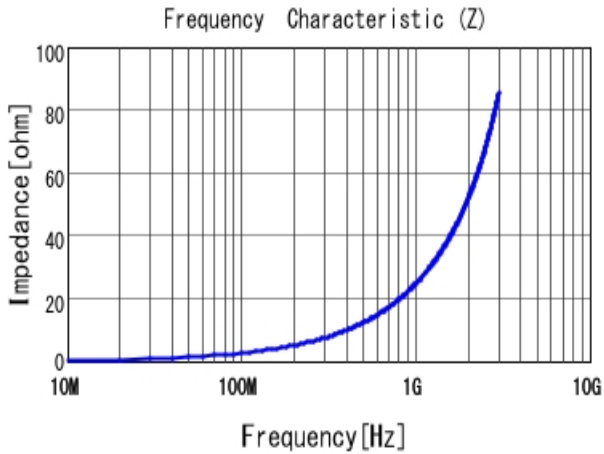
■ LQP03TN3N9B02 |Z|
