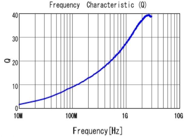
■ LQP03TN3N9B02 Q
