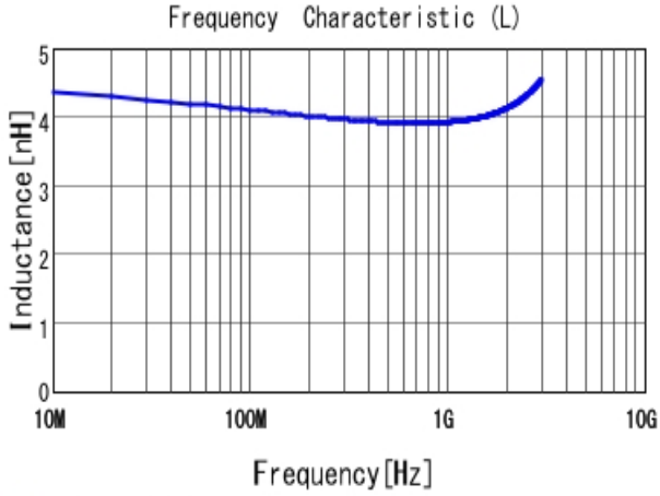
■ LQP03TN3N9B02 L
