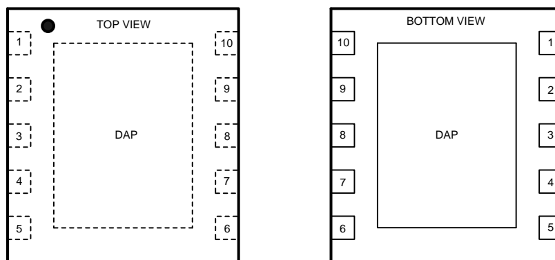
Figure 1. 10-Pin WSON (3mm x 3mm x 0.8mm)
