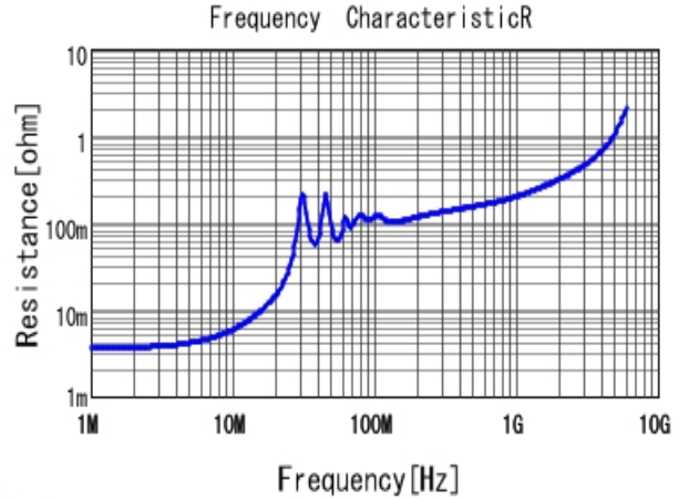
■ GRM31C5C1E104JA01 R DCOV, 25degC
