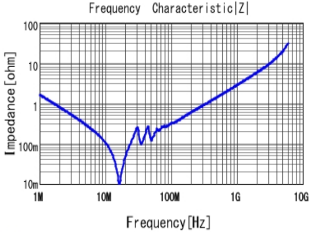
■ GRM31C5C1E104JA01 |Z| DCOV, 25degC
