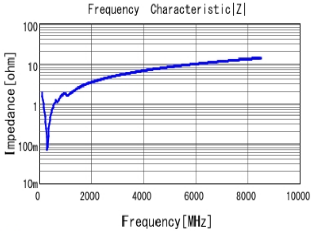
■ GRM1555C1H751GA01 |Z| DCOV, 25degC
