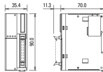
FC4A-D20K3, FC4A-D20S3
