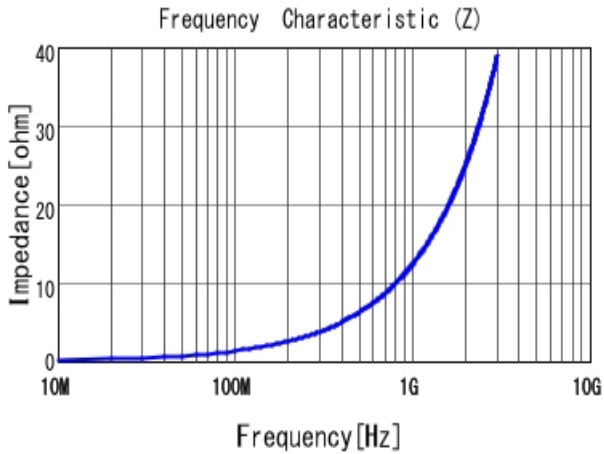
■ LQP03TN2N0B02 |Z|
