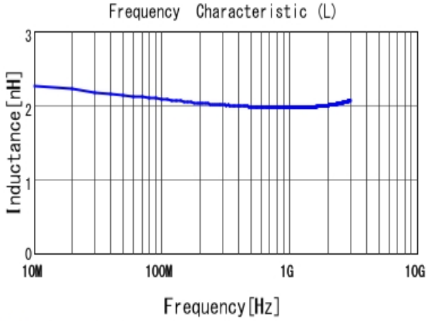
■ LQP03TN2N0B02 L
