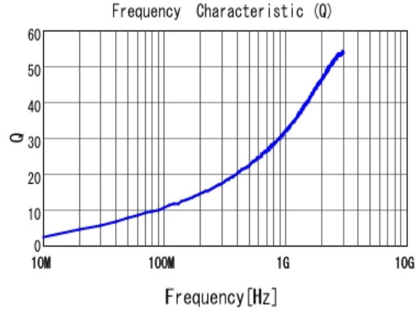
■ LQP03TN2N0B02 Q
