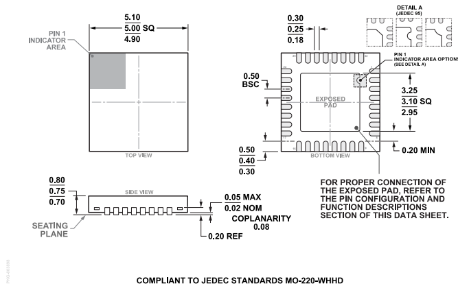
Figure 38. 32-Lead Lead Frame Chip Scale Package [LFCSP] 5 x 5 mm Body and 0.75 mm Package Height (CP-32-7) Dimensions shown in millimeters
