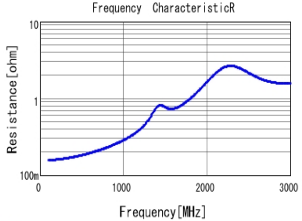
■ GRM21A7U2E101JW31 R DCOV, 25degC
