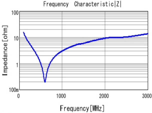
■ GRM21A7U2E101JW31 |Z| DCOV, 25degC
