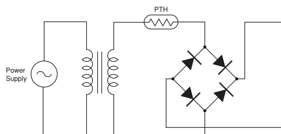
(3) Transformer Protection Circuit 2
