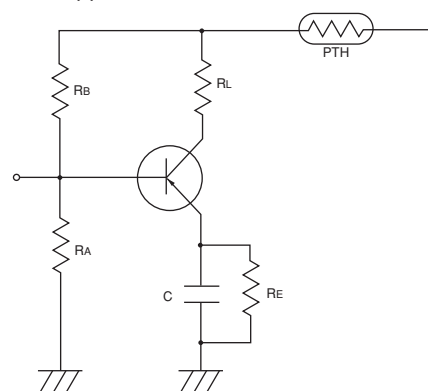
(1) Transistor Protection Circuit
