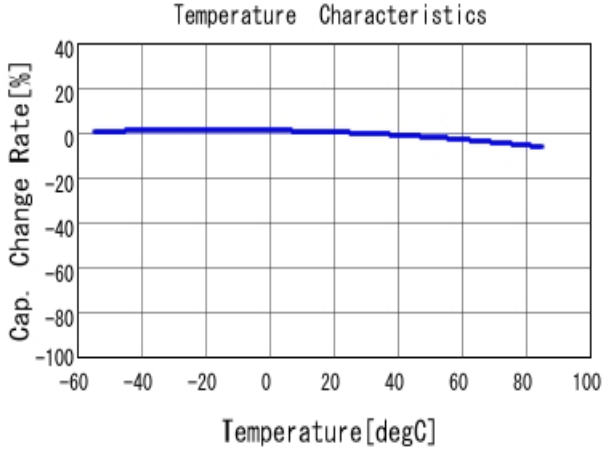
■ GRM188R61A334KA61 C-Temp. capchange, DC0.0V, AC1.0V r m
