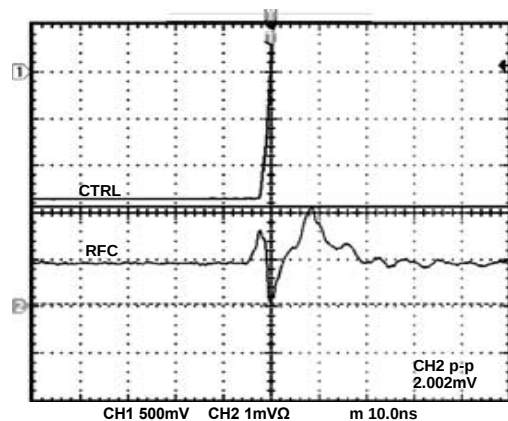
Figure 16. Video Feedthrough
