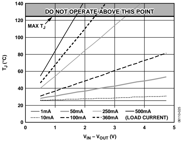
Figure 37. 0.70 mm 2 of PCB Copper, T A = 25°C
