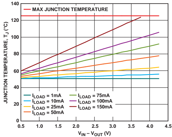
Figure 36. TSOT, 500 mm 2 of PCB Copper, T A = 50°C
