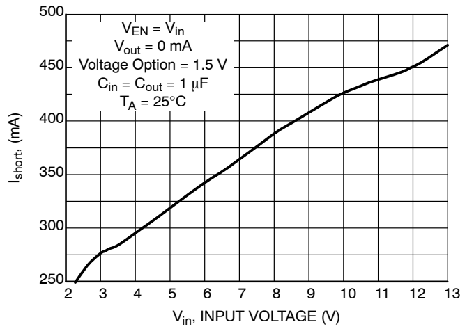
Figure 15. Output Short-Circuit Current vs. Input Voltage
