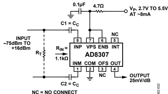
Figure 32. Basic Connections
