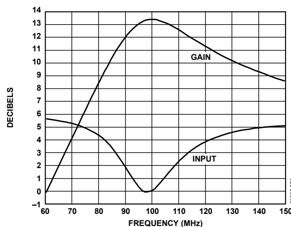
Figure 36. Response of 100 MHz Matching Network
