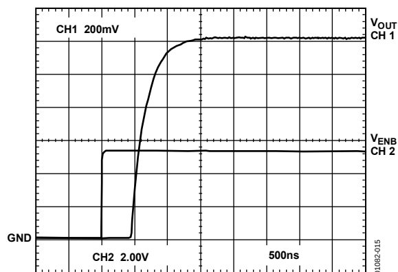
Figure 15. Power-Up Response Time
