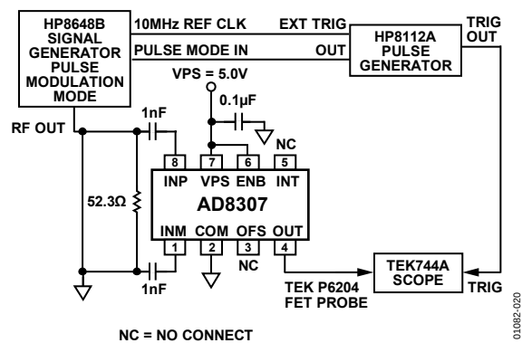
Figure 20. Test Setup for V_{OUT} Pulse Response
