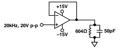
Figure 28. Output Swing, V_S = \pm 15V , G = +1
