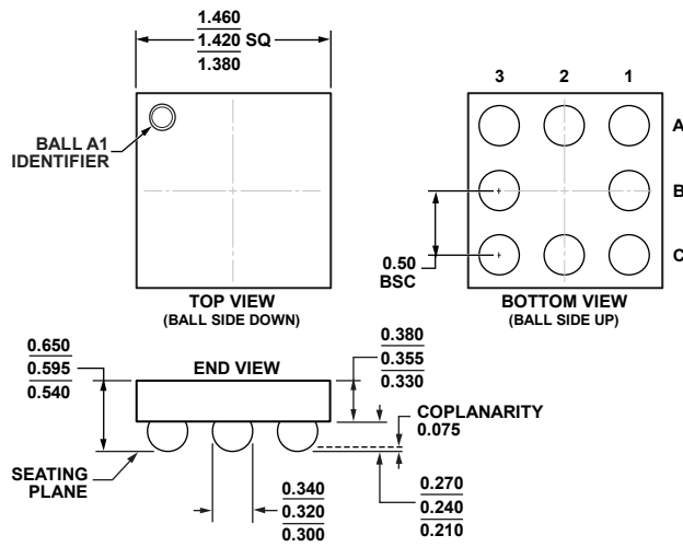
Figure 54. 8-Ball Wafer Level Chip Scale Package [WLCSP] (CB-8-2)
