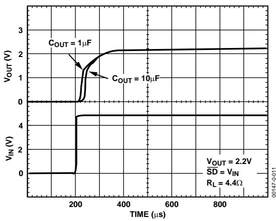
Figure 13. Power-Up Response
