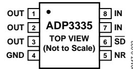
Figure 3. 8-Lead MSOP
