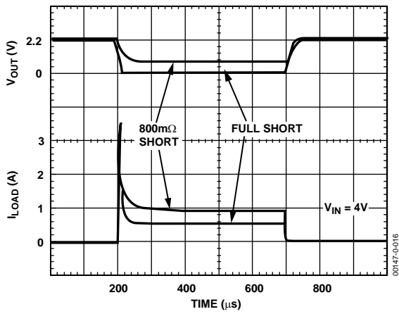
Figure 18. Short-Circuit Current
