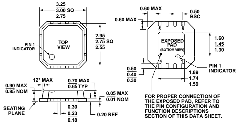
Figure 26. 8-Lead Lead Frame Chip Scale Package [LFCSF_VD] 3 mm × 3 mm Body, Very Thin, Dual Lead (CP-8-2) Dimensions shown in millimeters
