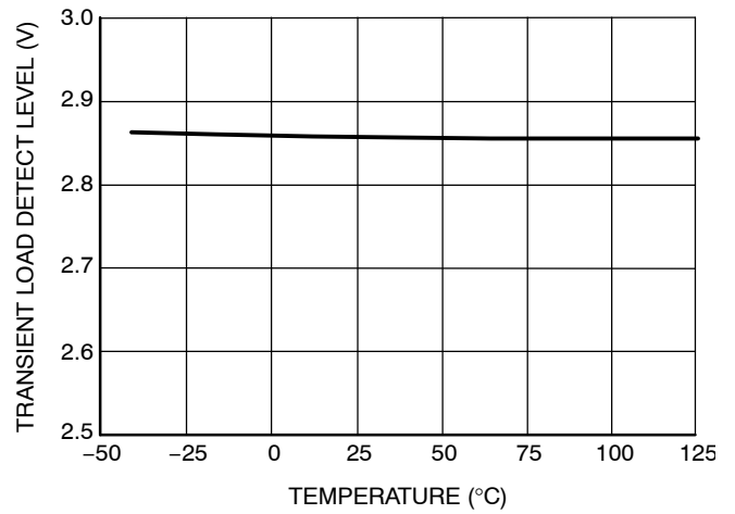
Figure 12. Transient Load Detect Level vs. Temperature
