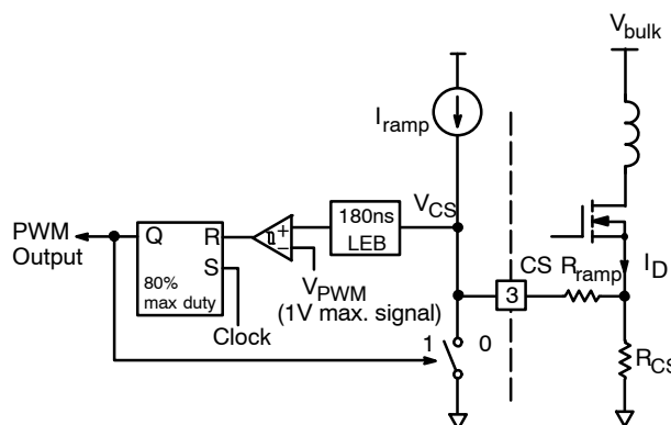
Figure 30. Current-Mode Implementation
