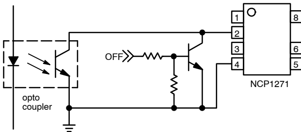
Figure 41. Non-Latchoff Shutdown
