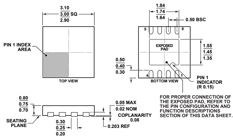
Figure 44. 8-Lead Frame Chip Scale Package [LFCSFP] 3 mm x 3 mm Body and 0.75 mm Package Height (CP-8-13) Dimensions shown in millimeters
