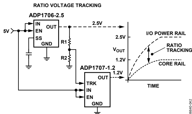
Figure 35. Voltage Tracking Feature Using the ADP1707
