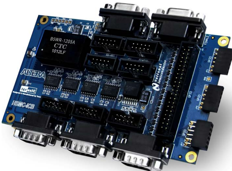
Figure 1-1 Layout of the ICB
