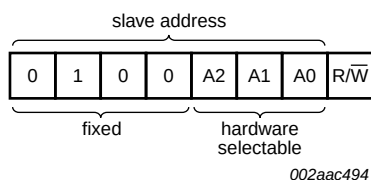
Fig 9. PCA9554 device address
