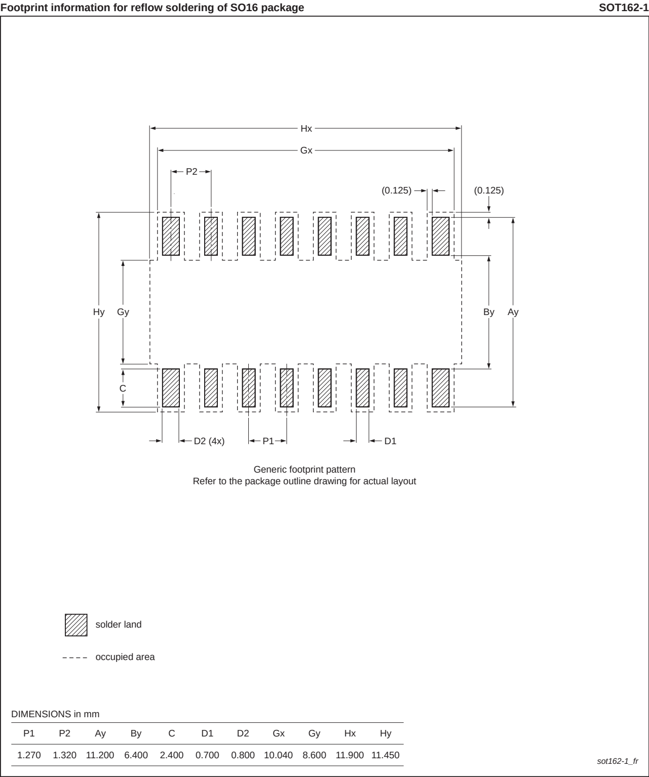
Fig 24. PCB footprint for SOT162-1 (SO16); reflow soldering
