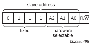
Fig 10. PCA9554A device address
