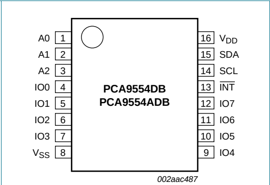
Fig 3. Pin configuration for SSOP16
