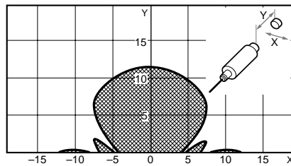
V600-D23P55 & V600-H52
