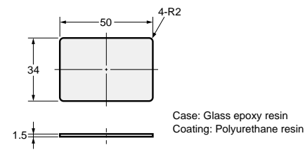
V600-D23P72
