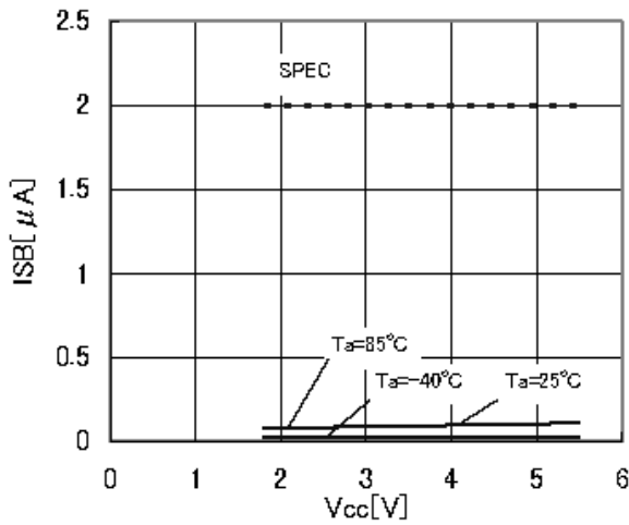
Figure 14. Standby current ISB
