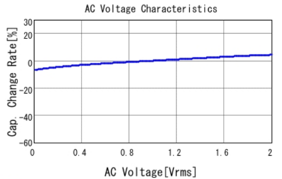
■ GCJ188R71C474KA12 C-AC Voltage capchange, DCOV, 25.0d
