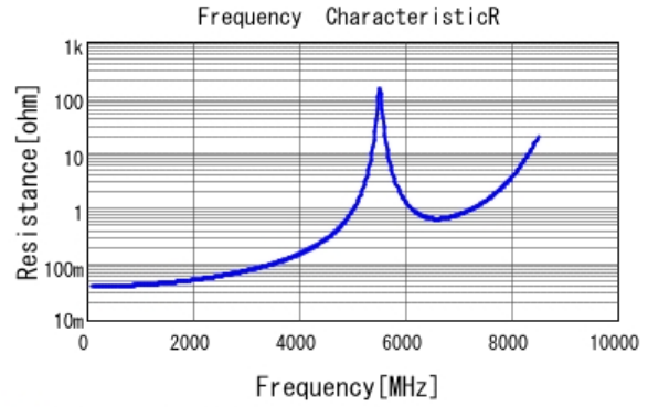
■ GQM2195C2E8R2CB12 R DCOV, 25degC
