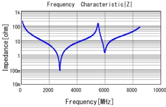
■ GQM2195C2E8R2CB12 |Z| DCOV, 25degC
