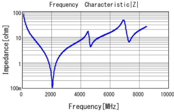
■ GJM1555C1H200JB01 |Z| DC0V, 25degC
