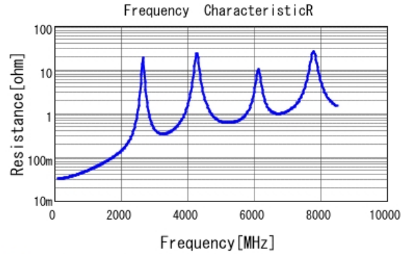
■ GQM1875C2E470JB12 R DC0V, 25degC
