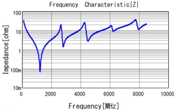
■ GQM1875C2E470JB12 |Z| DC0V, 25degC
