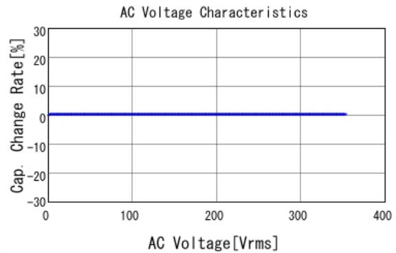
■ GRM31C7U3A102JW32 C-AC Voltage capchange, DCOV, 25.0d
