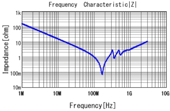
■ GRM31C7U3A102JW32 |Z| DCOV, 25degC
