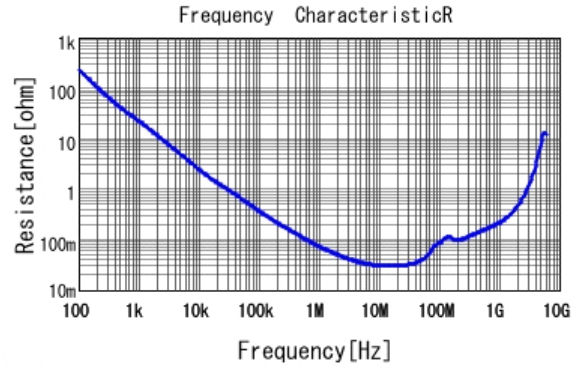
GCM188R71H333KA55 R DCOV, 25degC
