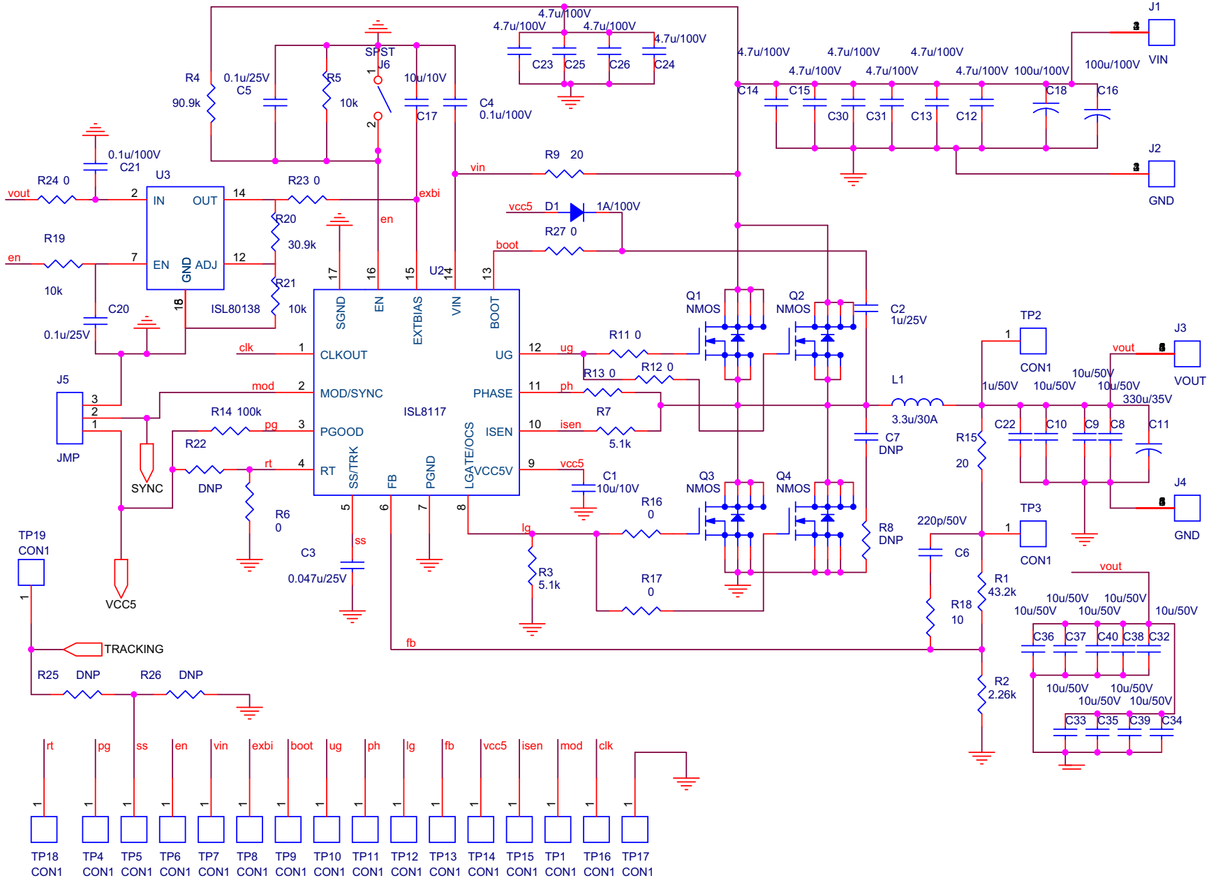
FIGURE 20. ISL8117EVAL2Z SCHEMATIC
