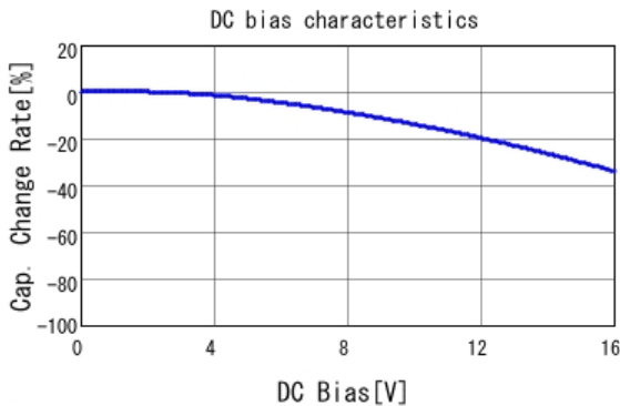
■ GRM188R71C334KA01 C-DC bias capchange, 25.0degC, AC1.
