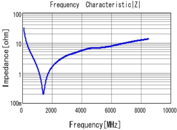
■ GRM0335C1H510GA01 |Z| DC0V, 25degC
