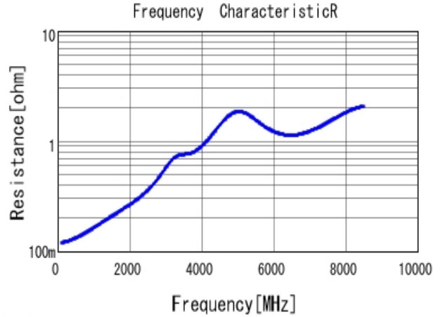
■ GRM0335C1H510GA01 R DC0V, 25degC
