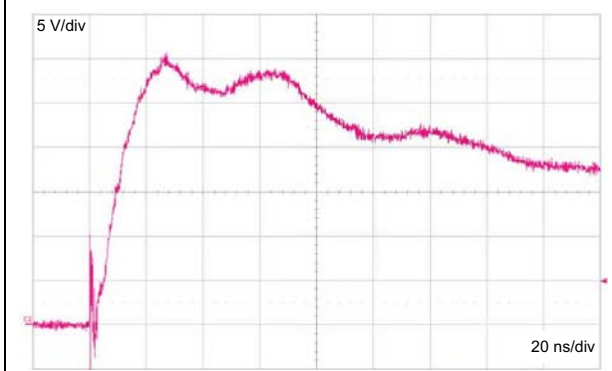
Figure 6. ESD response to ISO 10605- C = 330 pF, R = 330 \Omega (+15 kV contact)
