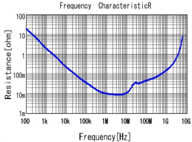
■ GCM188R71C474KA55 R DC0V, 25degC
