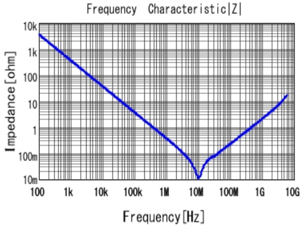
■ GCM188R71C474KA55 |Z| DC0V, 25degC
