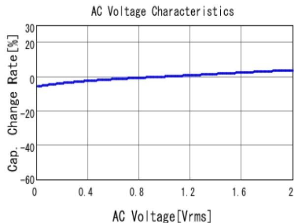
■ GCM188R71C474KA55 C-AC Voltage capchange, DC0V, 25.0d
