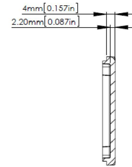
SECTION B-B SCALE 1 : 1
