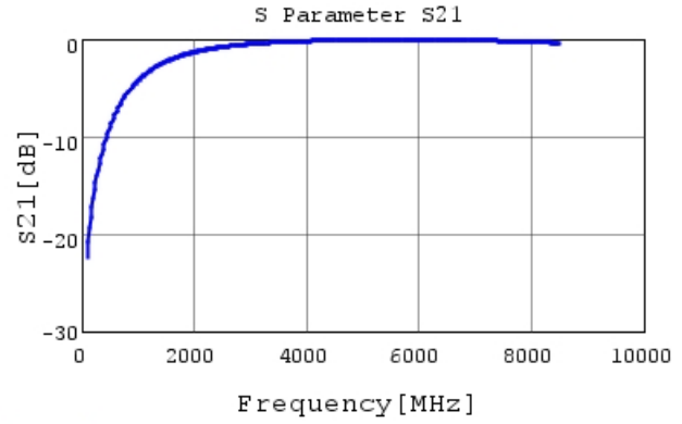
GRM1885C1H1R2BA01 S21 DCOV, 25degC
