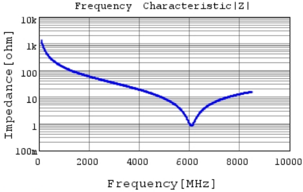
GRM1885C1H1R2BA01 |Z| DCOV, 25degC
