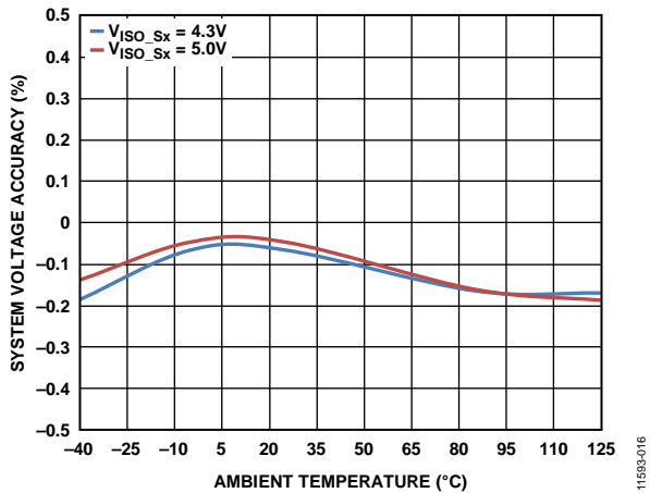
Figure 13. System Voltage Accuracy vs. Ambient Temperature, Load = 100 mA, V_{VINx} = 5.5V
