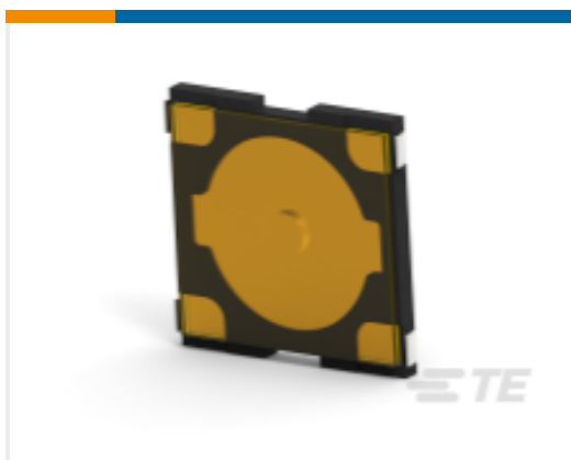
TE Part #2337233-5 TACT MICRO JB 4.8X4.8X0.55 P3.7 360GF
