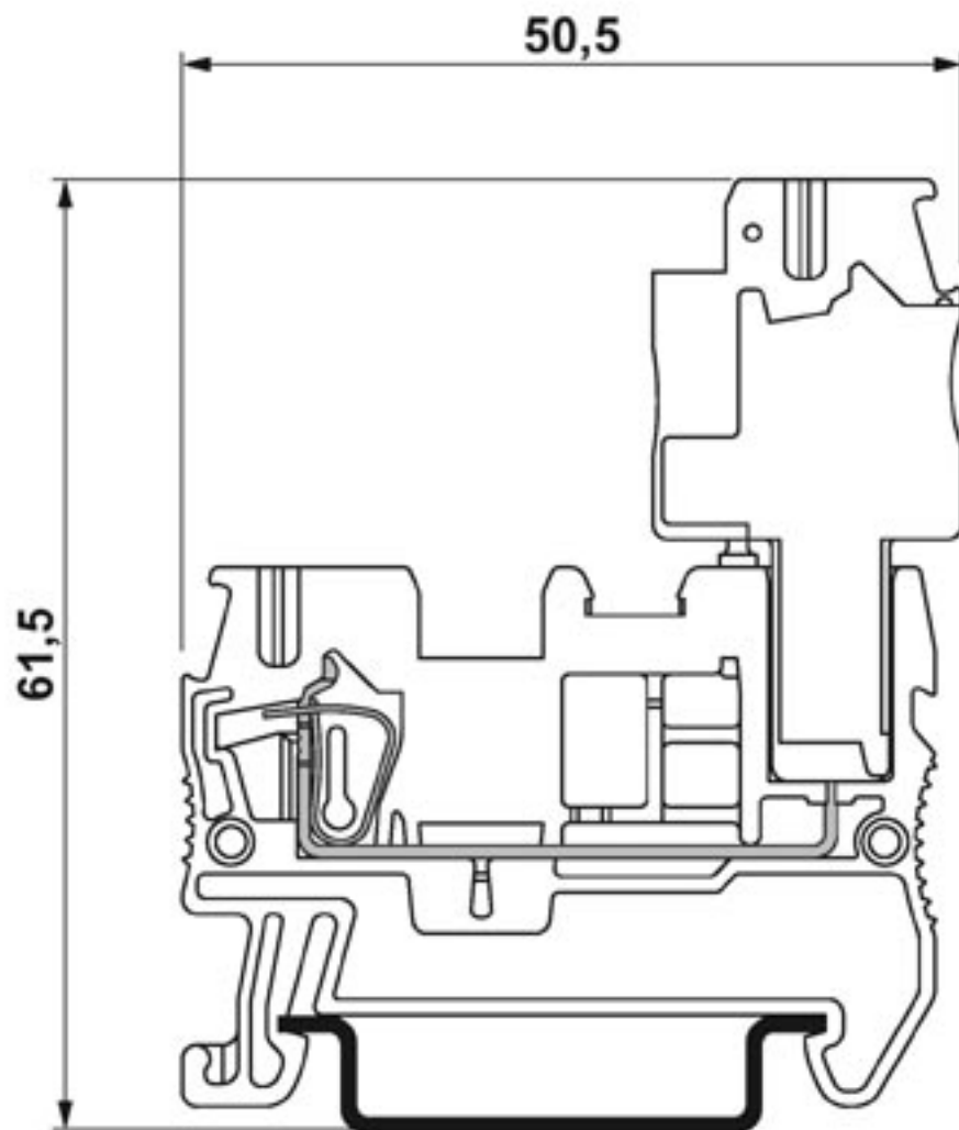
Dimensioned drawing
