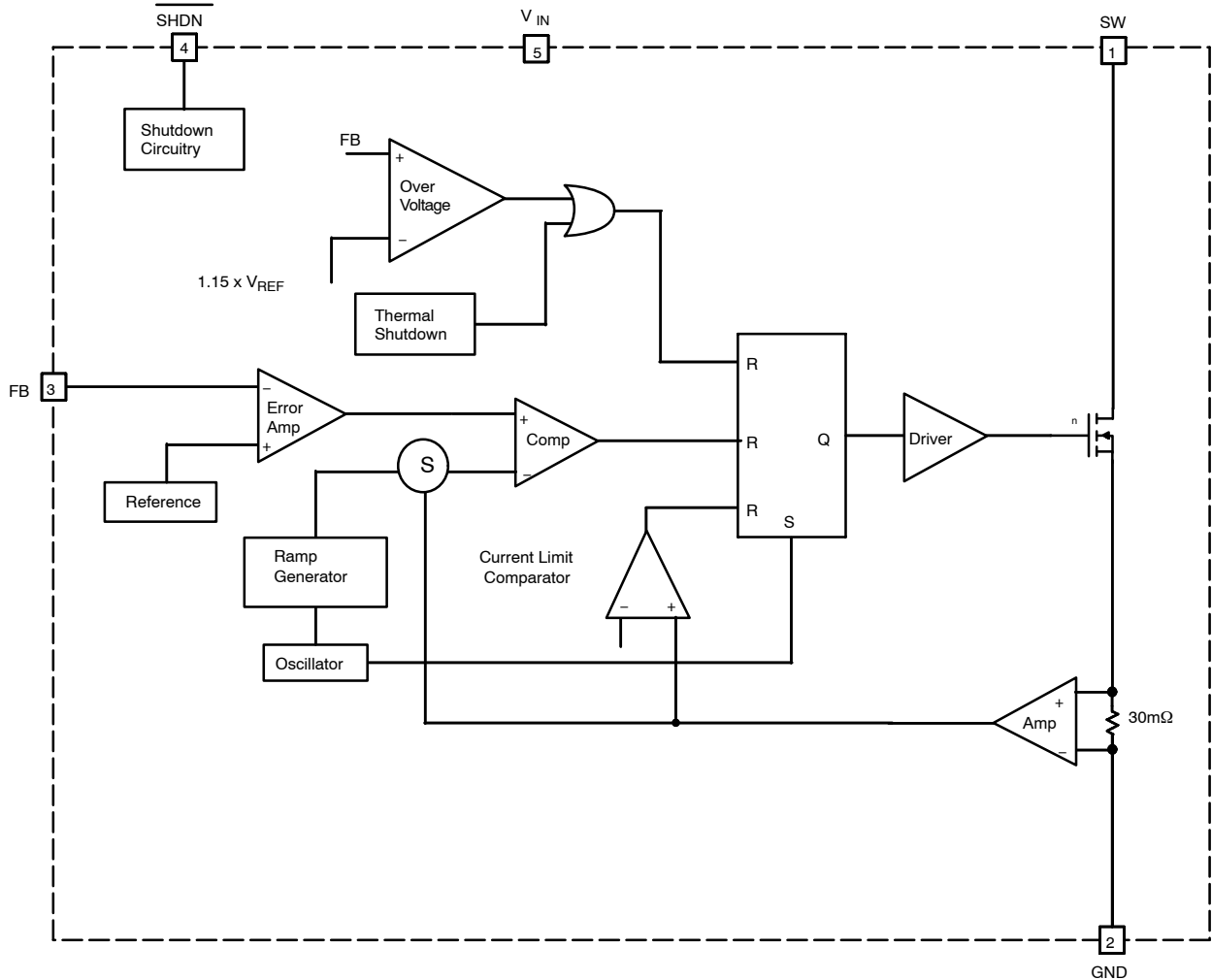
Figure 12. Block Diagram
