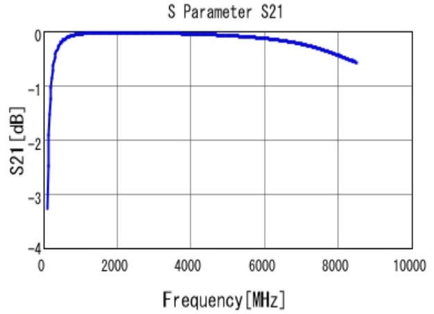
■ GRM0335C1E150JA01 S21 DCOV, 25degC
