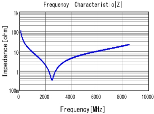
■ GRM0335C1E150JA01 |Z| DC0V, 25degC
