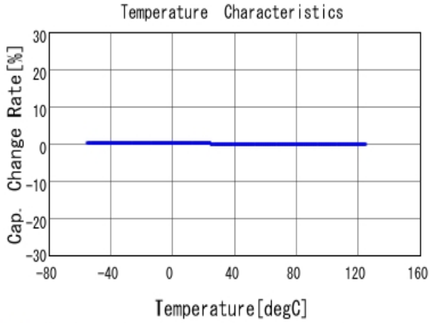
■ GRM0335C1E150JA01 C-Temp. capchange, DCOV, AC1Vrms
