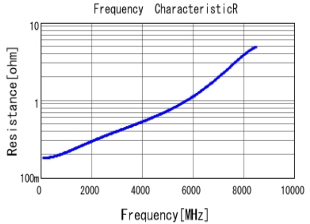
■ GRM0335C1E150JA01 R DC0V, 25degC
