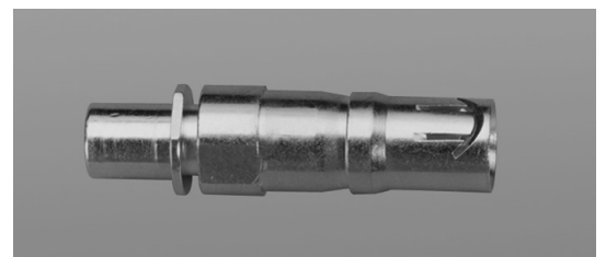
Socket Crimp Coax Contact for use in Miniature Crimp SE Type Connectors
