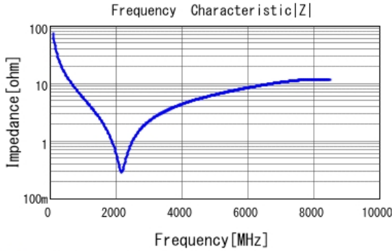
■ GRM0335C1H220JA01 |Z| DCOV, 25degC
