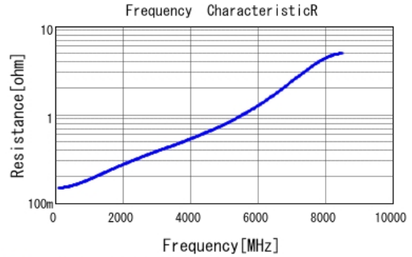
■ GRM0335C1H220JA01 R DCOV, 25degC
